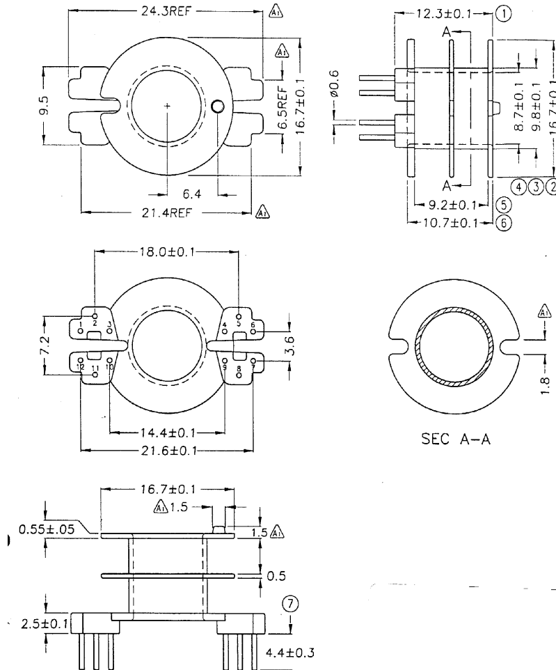
BOBBIN NAME: RM-8
