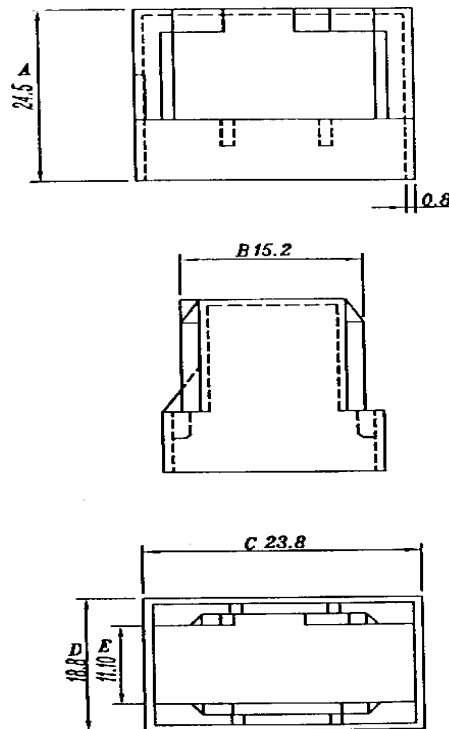
Series 4 Part No: BCEF20-CAP OLD REF: S174C1 Material: PBT/GF
