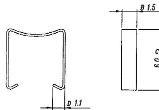
S4 Pt No: BCEE5-CLIP Material: SUS301 Old Ref: S096C5
