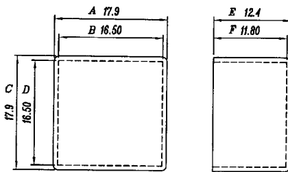
S4 Part No: BCEE16-CASE-2 Old Ref: S133C2 Material: PBT/GF
