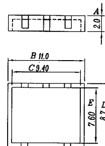
S4 Part No: BCEE16-CAP Old Ref: S133C3 Material: N46
