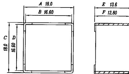
S4 Part No: BCEE16-CASE-1 Old Ref: S133C1 Material: PBT/GF
