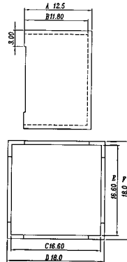
S4 Part No: BCEE16-CASE Old Ref: S133C Material: PBT/GF
