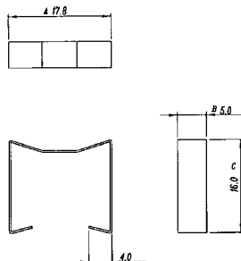
S4 Part No: BCEE16-CLIP Old Ref: S133C4 Material: SUS301 0.3t
